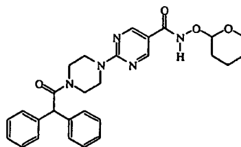
intermediate 7
